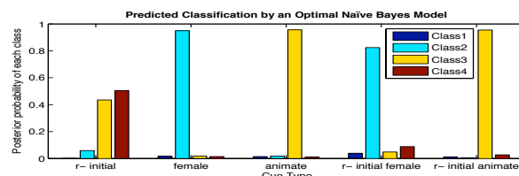
Figure 2: Predicted classification of novel nouns by an optimal naive Bayesian classifier
