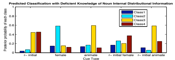
Figure 3: Classification of novel nouns as predicted by a Naïve Bayes Classifier with 95% of predictive semantic features misrepresented as [other].
