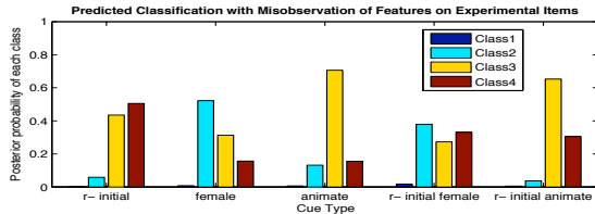
Figure 4: Classification of novel nouns as predicted by a model that misobserves semantic features on experimental items 58% of the time
