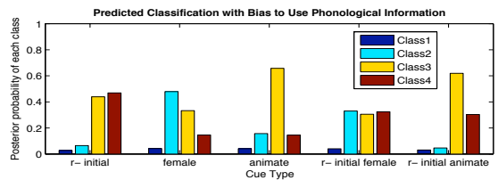
Figure 5: Classification as predicted by a model biased not to use semantic information 65% of the time
